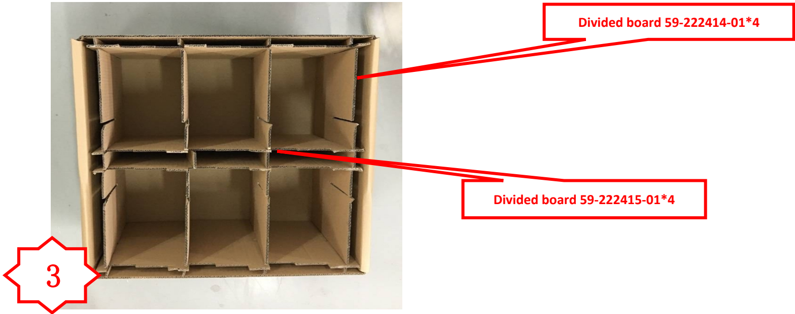
Assemble the two types divided board and put it in inner box second
